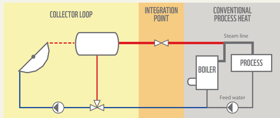
Figure 7: Direct solar steam generation
