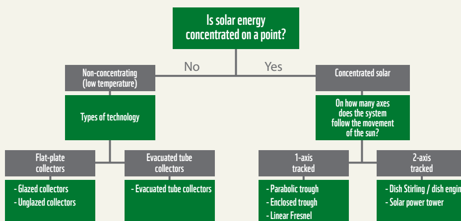
Figure 4: Range of solar collectors
