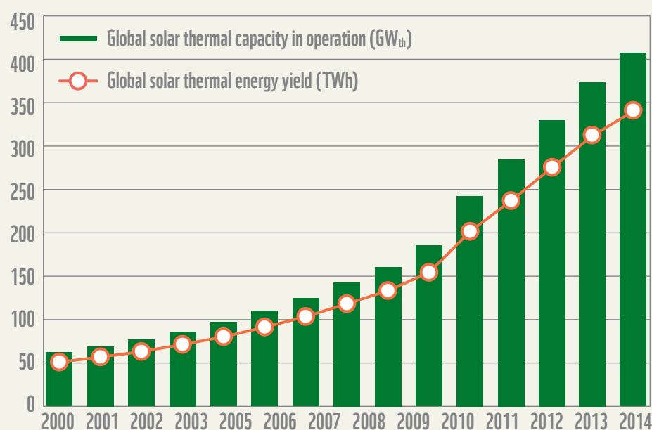
Figure 11: Global solar thermal capacity in operation and annual energy yields 2000–2014
