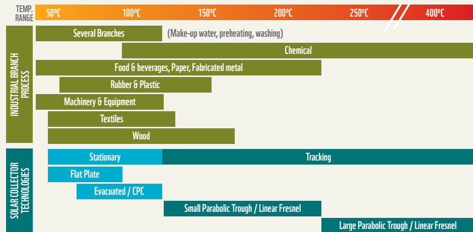
Figure 10: Stationary and tracking solar collector technologies related to operation temperature and process temperature range in different industrial branches
