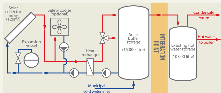
Figure 16: A schematic of Migra's system
