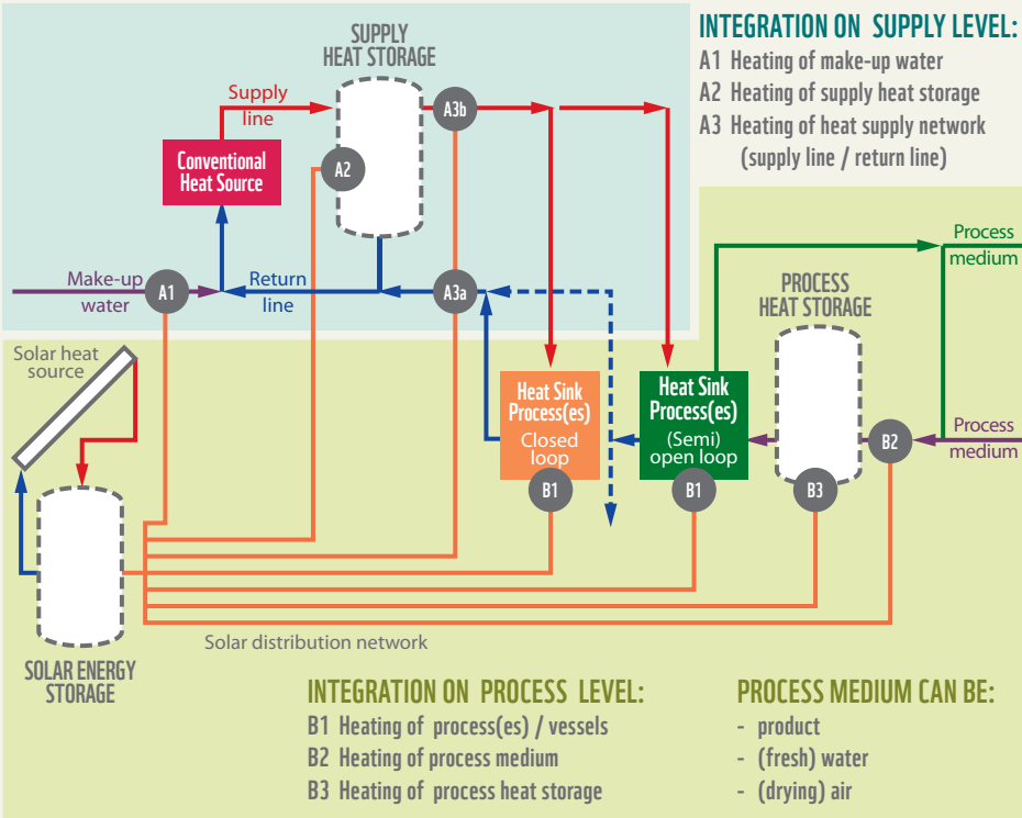
Figure 8: Possible integration points for solar process heat
