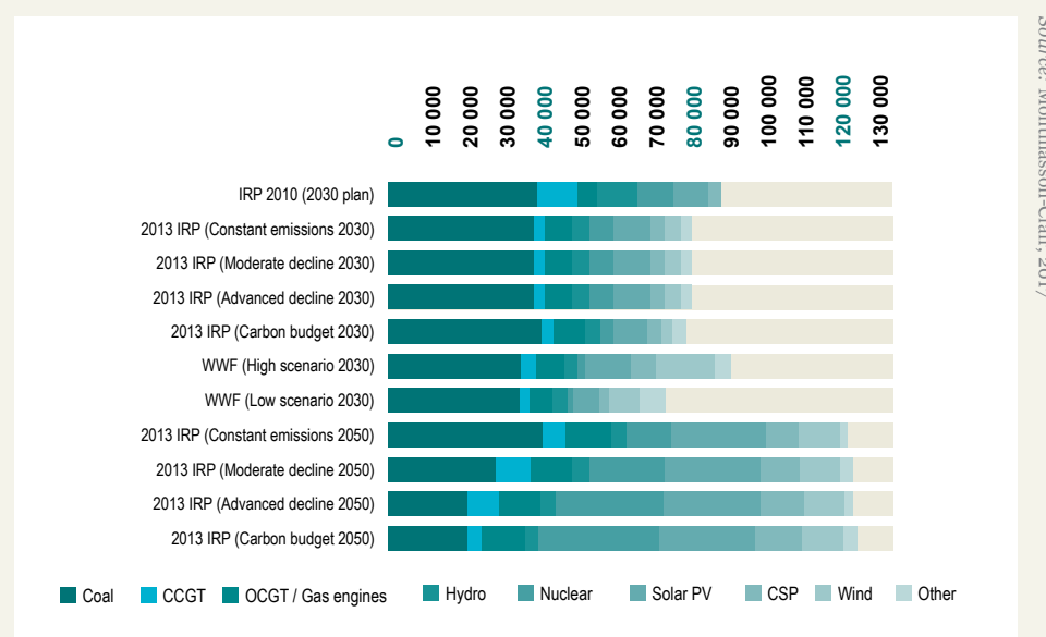
Figure 3.2: Electricity mix (in MW of generation capacity) in 2030 and 2050 according to different scenarios
